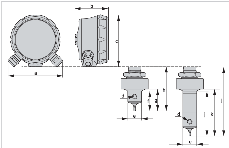
Figure 2-1: Dimensions
